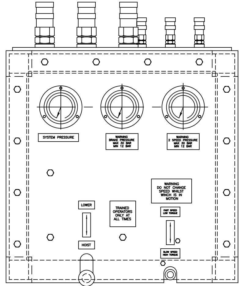
ENLARGED LAYOUT OF CONTROLS & LABELS.
